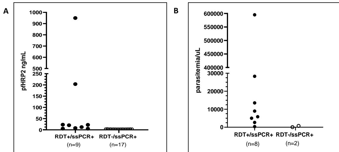
Supplemental Figure S2. (A) Plasma PfHRP2 levels and (B) Peripheral parasitemia, in RDT+/ssPCR+ vs. RDT-/ssPCR+ sample subsets
