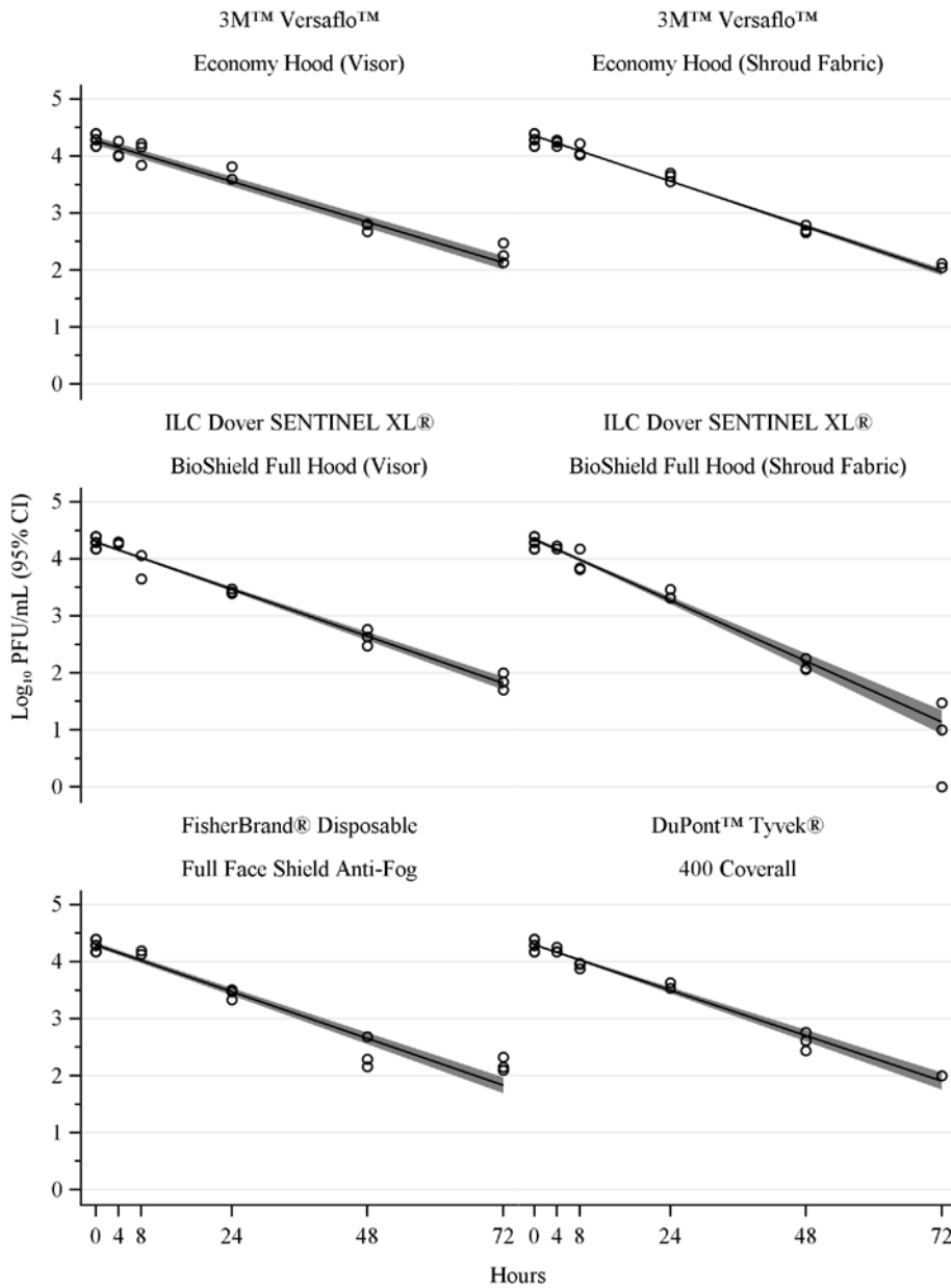
Geometric mean half-life of SARS-CoV-2 on Personal Protection Equipment (PPE). The line indicates the estimated mean titer, with bands extending to the 95% Confidence Interval. Estimates are based on an over-dispersed Poisson generalized estimating equation. Points indicate individual observations. Observations of 0 PFU are plotted at 0.01 PFU/mL.
